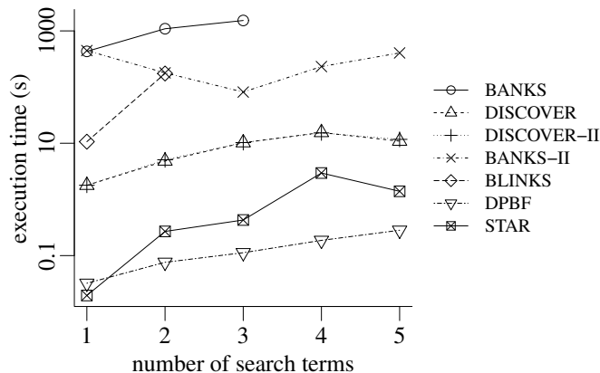
Fig. 4. Mean execution time vs. query length; lower execution times are better. Note that the y -axis has a log scale. The retrieval depth was 100 results.
