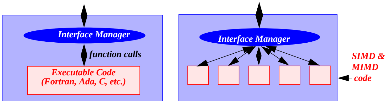
Figure 1: Object wrappers.
