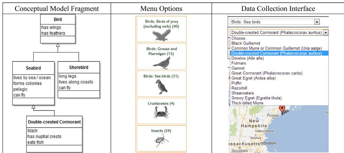
Fig. 1. Connection between a conceptual modeling fragment (showing how birds are classified per requirements of the scientists) and user interface design in Phase 1 of NLNature.
