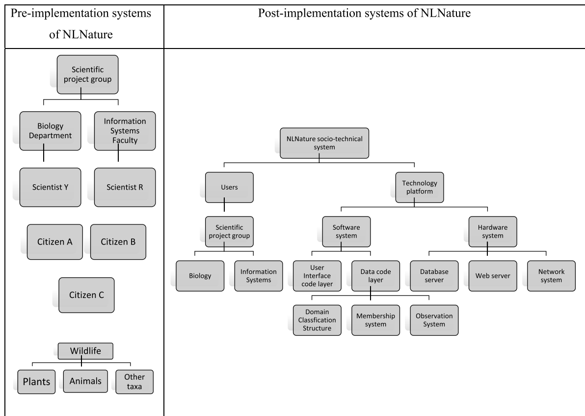
Fig. 6. Level Structure Models of pre-NLNature systems (left) and NLNature socio-technical system (right) (adapted formalism from [75]); boxes represent systems at different levels; lines represent composition relationships. Note: in NLNature user interface and data code layers were designed as separate and interacting subsystems, to permit implementation on multiple devices.
