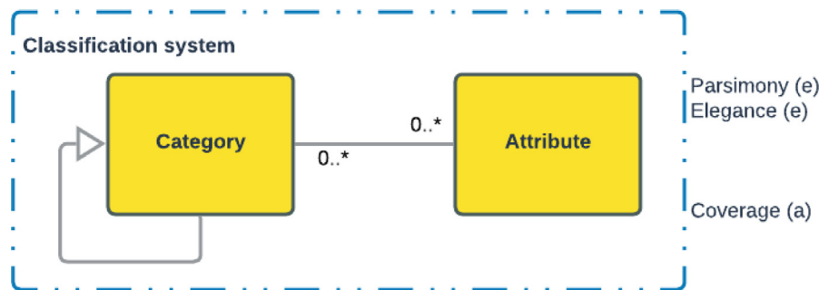
Fig. 8. Modeling a system by extending UML grammar to distinguish aggregate (a) and emergent (e) properties.
