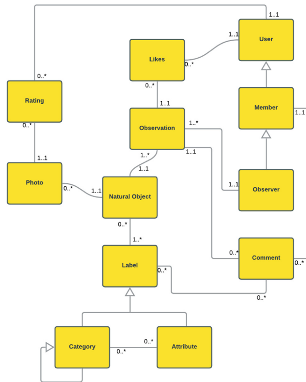
Fig. 3. A conceptual model in Phase 2 of NLNature. . (For interpretation of the references to color in this figure legend, the reader is referred to the web version of this article.)
