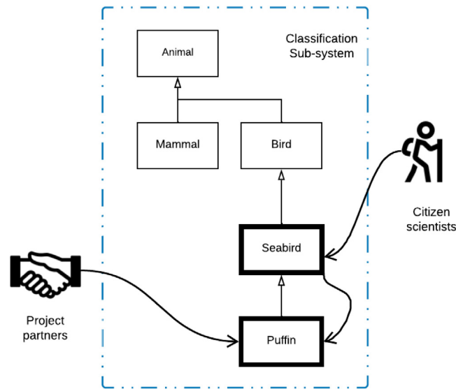
Fig. 4. Example of a System Boundary Model (SBM) fragment. Classification structure as a conceptual system (call-out bubble); boundary objects of system shown as classes with bold outlines; important environment objects shown as icons of citizen scientists and project partners.
