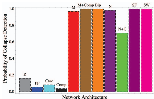
Figure 4. Distribution of the correlation, \rho_K , between \text{Max}[S_y] and the parameter p , after 1000 realizations for the full disordered (not mean-field) case. If \rho_K is significant ( p -value < 0.05 ) and \rho_K > 0.5 the increase in \text{Max}[S_y] is interpreted as an early warning sign. We calculate these detection statistics for several realizations of each network structure and determine the probability of detecting the early warning sign of instability. We consider eleven different network architectures typical of ecological or social networks, including random (R), predator-prey (PP), cascade (Casc), compartmentalized (Comp), mutualistic (M), bipartite (Bip), nested (N), nested with competition (N+C), scale free (SF), and small world (SW). These networks have different structures for the adjacency matrix and different combination of interaction types, i.e. (++) mutualistic, (+-) antagonistic, (--) competitive or a combination of them (See Materials S1 for more details). doi:10.1371/journal.pone.0101851.g004
