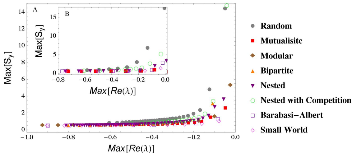
Figure 2. \text{Max}[S_y] as a leading indicator of instability in a “mean field” network with constant interaction intensity (in absolute value), p . Instability is attained by increasing p (main panel A, with N=20 , C=0.2 ) or C (inset B, with N=20 , and C increasing from 0.1 to 1) with different network structures. The figures represent average behavior over 1000 realizations. doi:10.1371/journal.pone.0101851.g002
