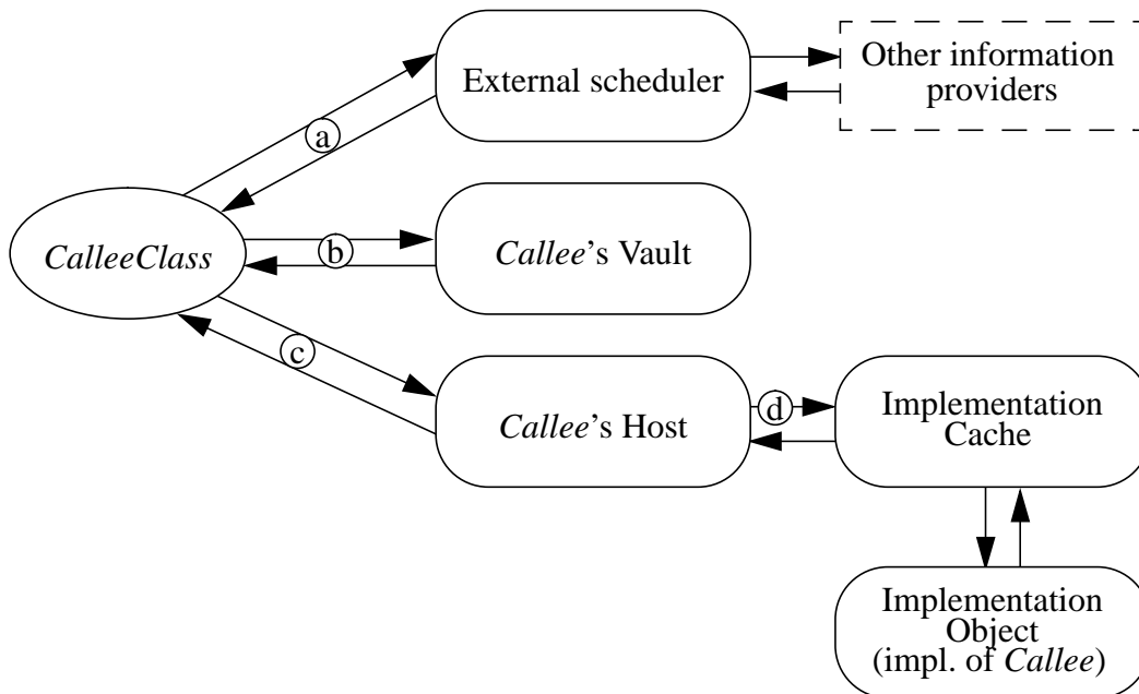
FIGURE 7. The Legion object activation mechanism—CalleeClass wishes to activate Callee. First, CalleeClass must decide on which host and vault to place Callee. To do this, CalleeClass may consult an external scheduler (a). After a placement decision is made, CalleeClass must determine the OPA for Callee by consulting Callee's vault (b). Finally, to activate Callee, CalleeClass sends an activation request to the desired host (c) specifying the object LOID, implementation to use, and OPA. To create a process for Callee, the host must obtain the implementation for Callee. To do this, the host uses a shared implementation cache object (d). After downloading the implementation, the host starts a process for Callee and returns the binding to CalleeClass.
