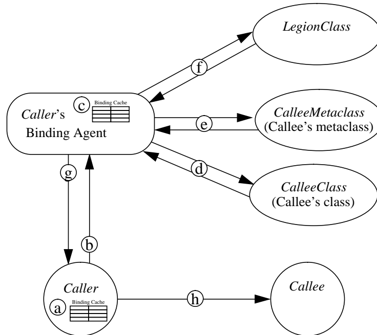
FIGURE 6. Potential steps in the Legion binding and class-of mechanisms—Caller must bind the LOID of Callee to an OA for low-level communication. Caller may already have a cached binding for Callee (a), or may need to consult a binding agent (b). The binding agent may have a cached binding for Callee (c), or may need to consult Callee’s class, CalleeClass , for the binding (d). In order to communicate with CalleeClass , the binding agent needs a binding for CalleeClass . If the binding agent does not have CalleeClass ’s binding, it may need to consult CalleeClass ’s metaclass (e). If the binding agent does not know the binding for this metaclass, the process repeats itself. The recursion is guaranteed to terminate at the root of the binding tree, LegionClass (f). Eventually, the binding agent returns Callee’s binding (g) and Caller can send messages directly to Callee (h).
