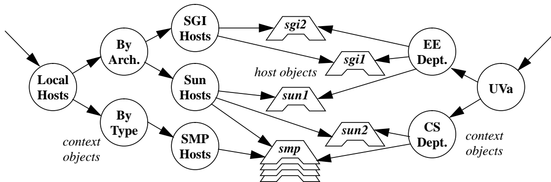
FIGURE 17. Context space used to organize information about host objects
