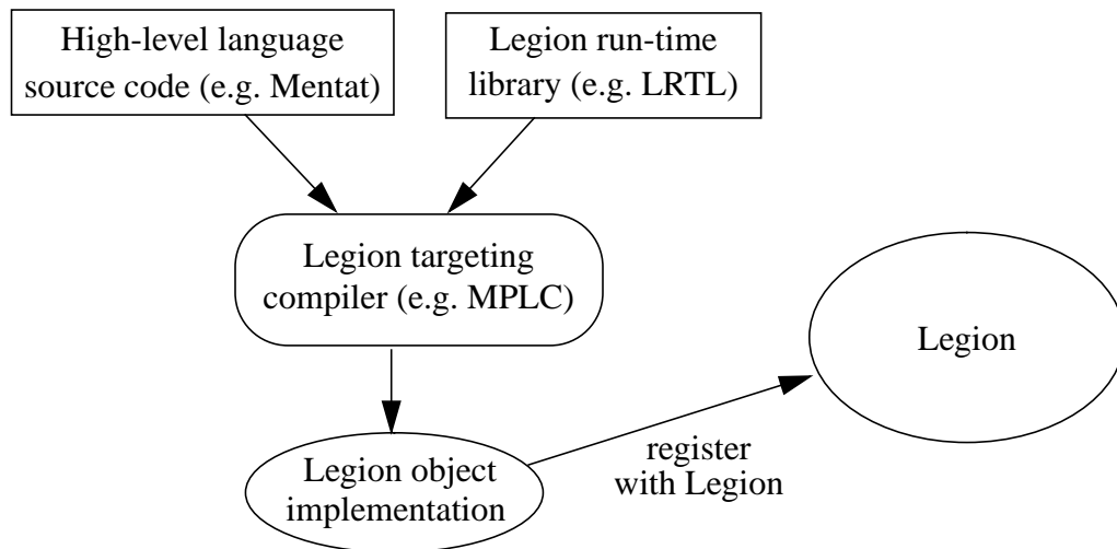
FIGURE 4. The Legion programming model. The object is defined in a high level language. Through a combination of Legion-aware compiler support and use of the LRTL, a complete Legion object implementation is produced. Based on this object implementation, new Legion objects can be instantiated in the system. These new objects can communicate with one another and with existing Legion objects.
