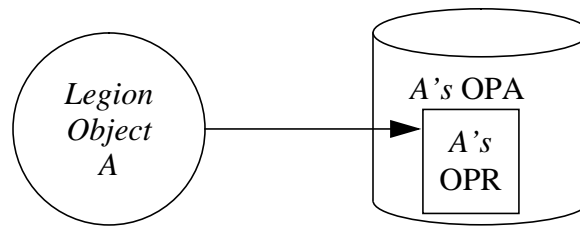
FIGURE 3. A Legion object has direct access to its persistent state, termed its object persistence representation, or OPR. The location of an object's OPR is called the object persistence address, or OPA.
