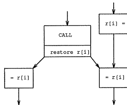
Figure 4. Use Preceded by a Set
