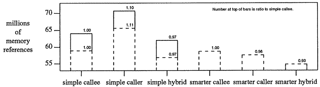
Figure 11. Total Memory References Performed - Motorola 68020
