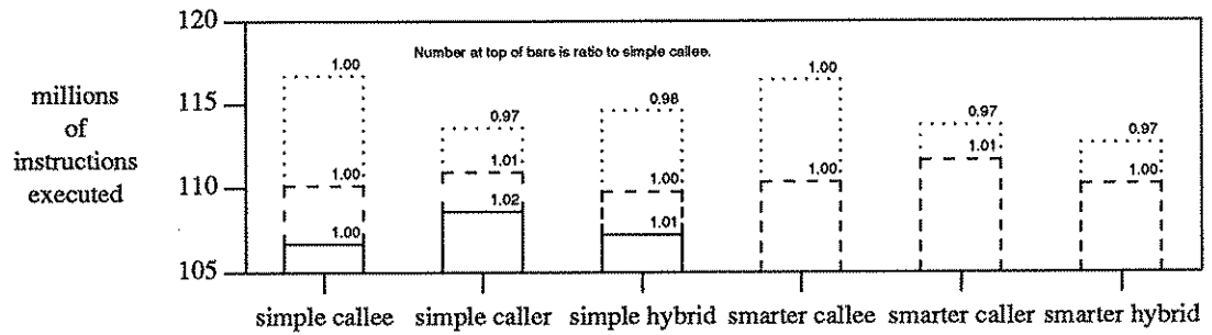
Figure 7. Total Instructions Executed - VAX-11
