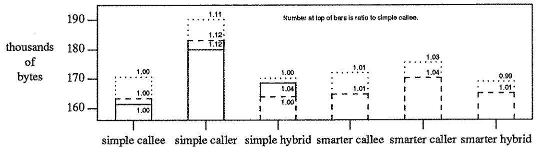
Figure 12. Static Code Size - Motorola 68020
