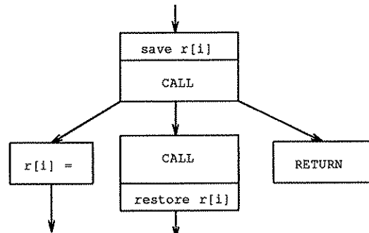
Figure 2. Only Sets, Calls, and Returns after Call
