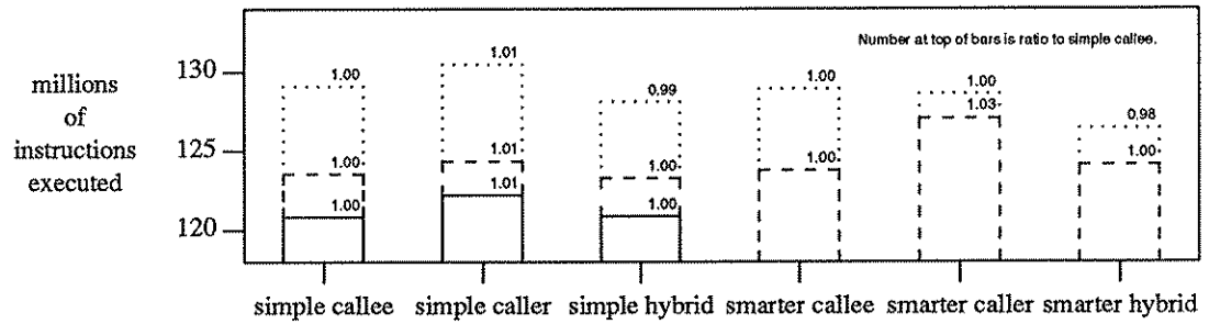
Figure 10. Total Instructions Executed - Motorola 68020
