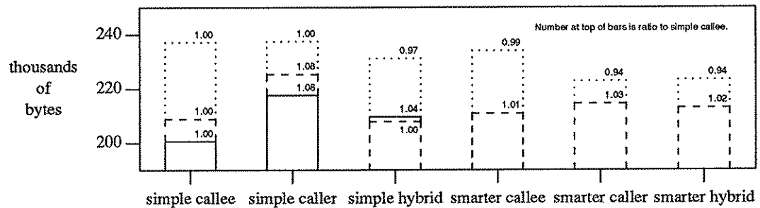
Figure 9. Static Code Size - VAX-11
