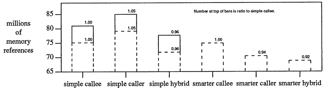
Figure 8. Total Memory References Performed - VAX-11
